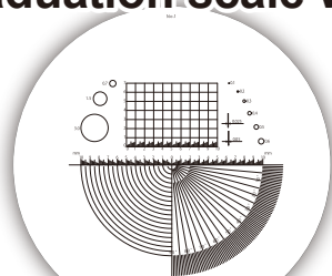
■ NLSL-10-1 / NLSL-15-1 Scale line image
